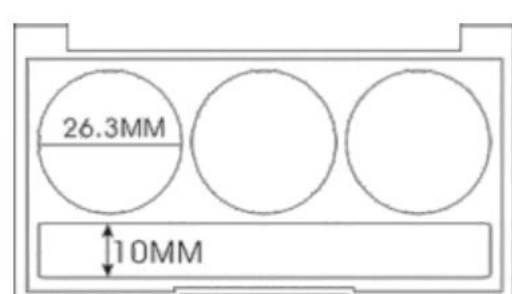
HG7169B SIZE:L91.4*W51*H11.5MM
