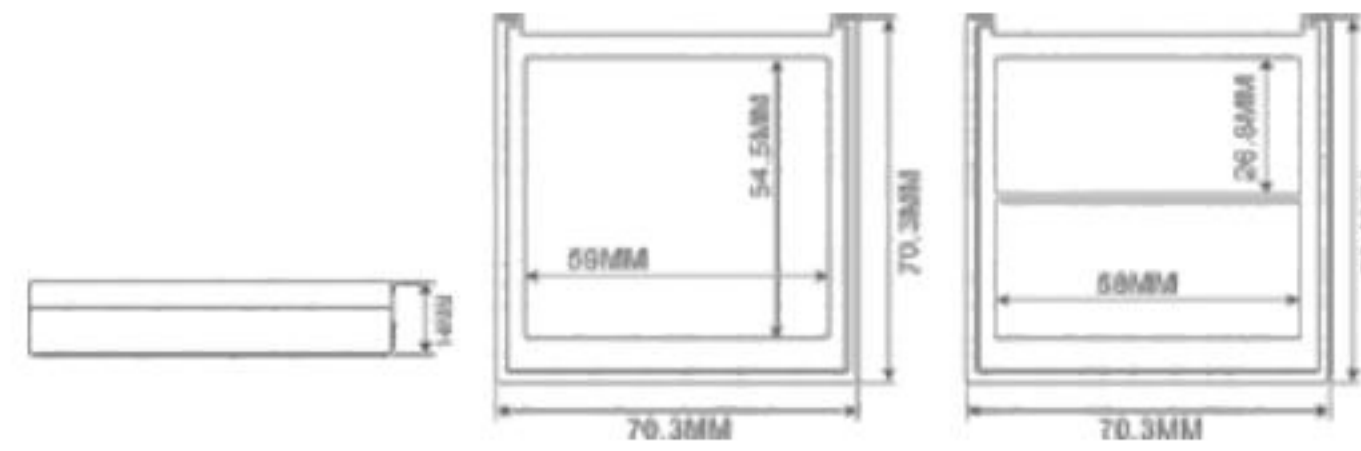
HG7236A SIZE:W70.3*H14MM
