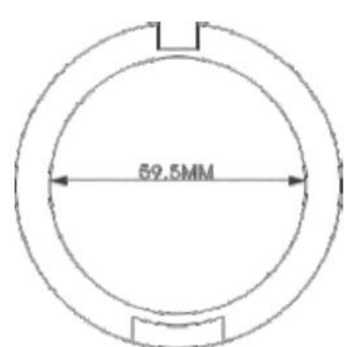
HG7075 SIZE:W67.7*H25.5MM
