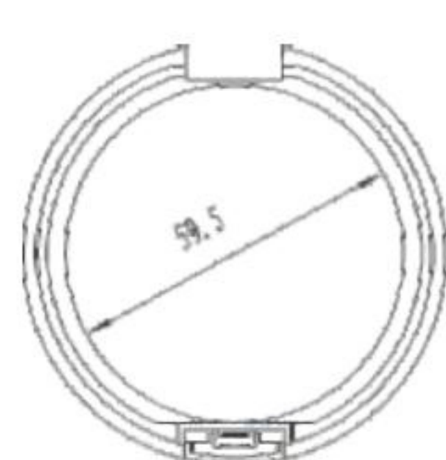
HG7111A SIZE:W76.5*H22MM
