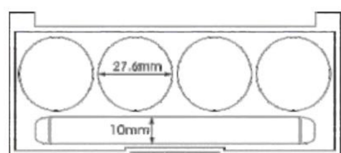
HG7080A SIZE:L124*W54*H14.6MM
