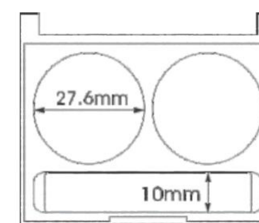
HG7081A SIZE:L64*W54*H14.6MM
