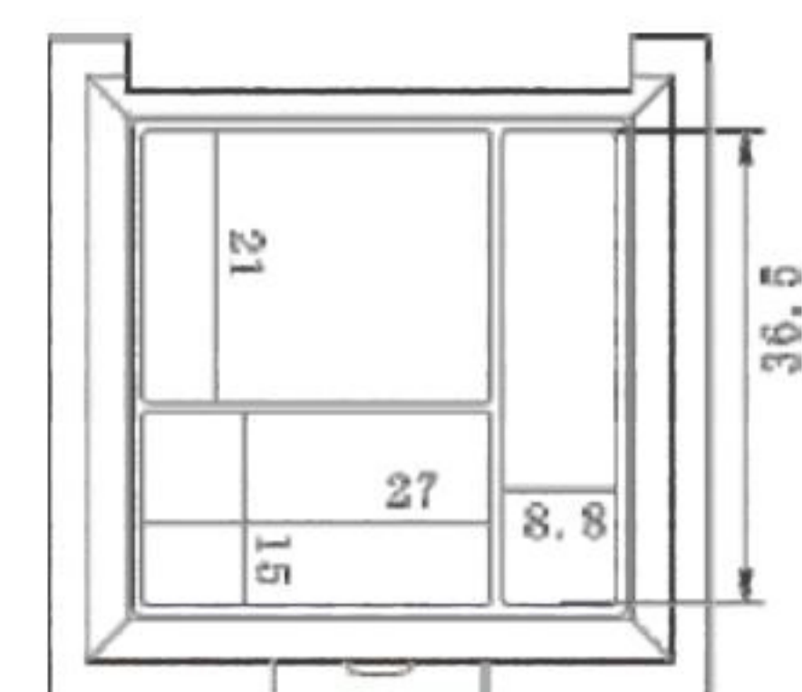
HG7181B SIZE:L51.7*W51.7*H15.6MM
