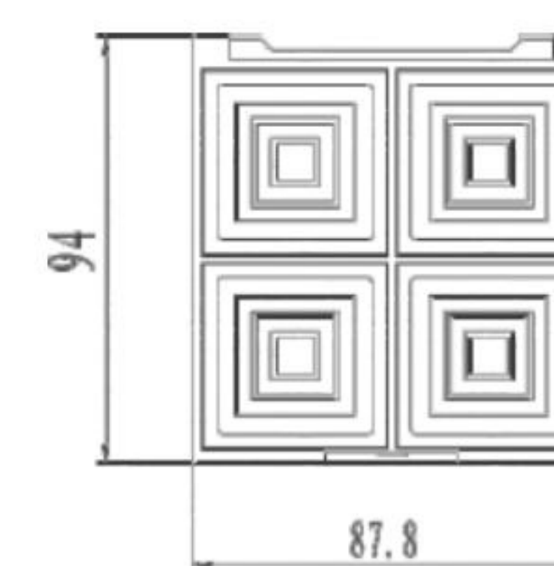
HG7089 SIZE:L93.5*W87.5*H13.5MM
